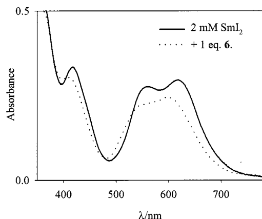
Figure 4. UV-vis spectra of \text{SmI}_2 in THF ( 2 \times 10^{-3} M) alone and with 1 equivalent of 6 added
