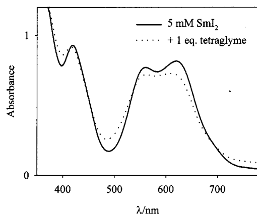
Figure 1. UV-vis spectra of \text{SmI}_2 in THF ( 5 \cdot 10^{-3} M) alone and with 1 equiv. of tetraglyme added
