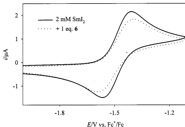
Figure 5. Cyclic voltammograms of \text{SmI}_2 recorded with 0 and 1 equivalents of 6 added; 2 \cdot 10^{-3} M \text{SmI}_2 in THF/ 0.2 M n\text{Bu}_4\text{NPF}_6 + 0.02 M n\text{Bu}_4\text{NI} ; electrode material: glassy carbon; sweep rate: 100 mV/s.
