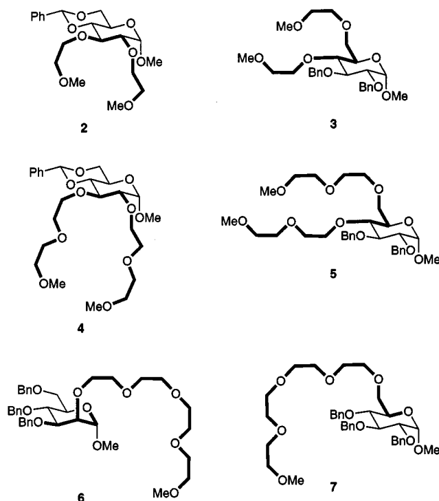
Figure 3. Various carbohydrate polyethylene glycol derivatives tested for in the \text{SmI}_2 -promoted pinacol coupling
