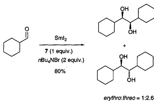
Scheme 1. Pinacol coupling reaction of cyclohexanecarboxaldehyde with the \text{SmI}_2/n\text{Bu}_4\text{NBr}/\mathbf{7} combination
