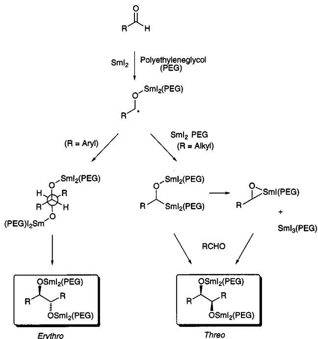
Scheme 3. Mechanistic proposal for the pinacol coupling reaction induced by PEG-complexed \text{SmI}_2 .
