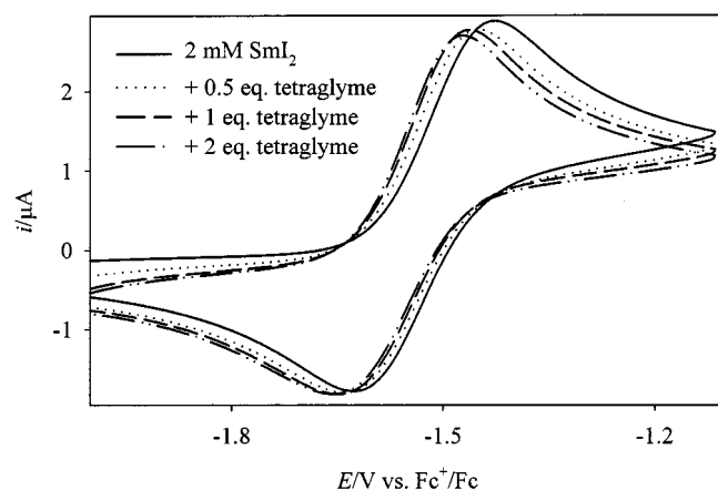
Figure 2. Cyclic voltammograms of \text{SmI}_2 recorded with 0, 0.5, 1 and 2 equivalents of tetraglyme added; 2 \cdot 10^{-3} M \text{SmI}_2 in THF/0.2 M n\text{Bu}_4\text{NPF}_6 + 0.02 M n\text{Bu}_4\text{NI} ; electrode material: glassy carbon; sweep rate: 100 mV/s.
