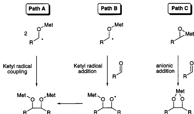
Scheme 2. Proposed mechanisms for the transition metal-promoted coupling pinacol reaction
